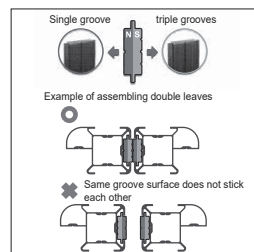
Aluminum opening/closing fitting with a handle for double leaves (Detailed drawing of the magnet surface)
